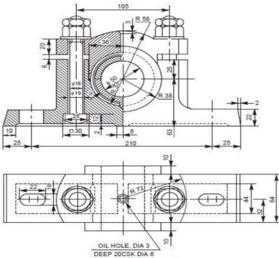
Fig. 12.4 Plummer block
