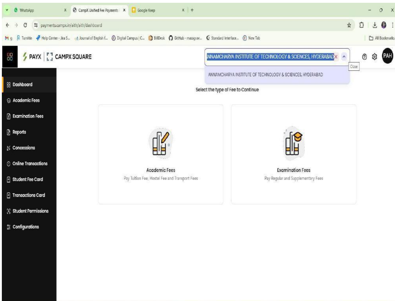
Dashboard Screenshot
